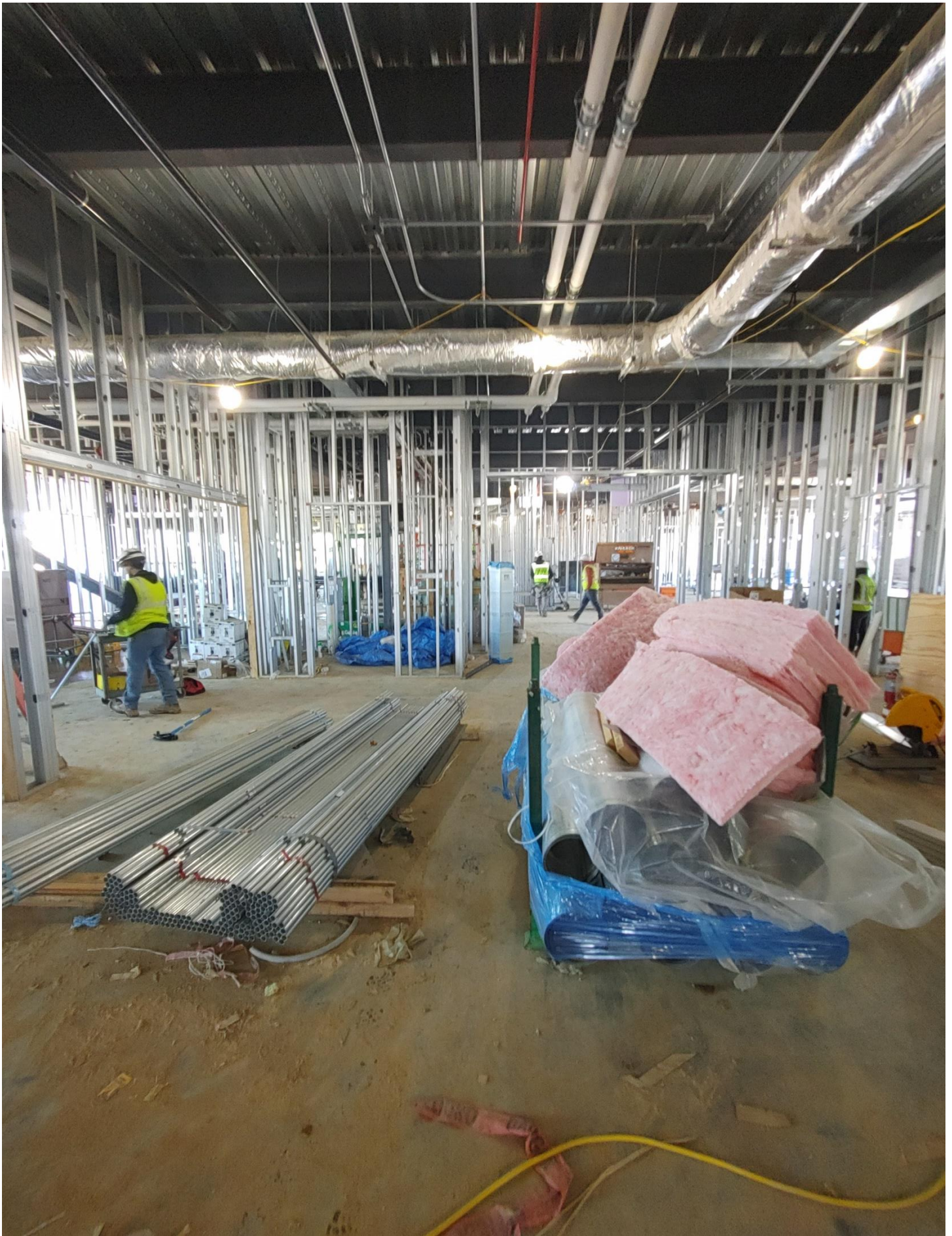
Photo 7 - Framing continues in Area B.
