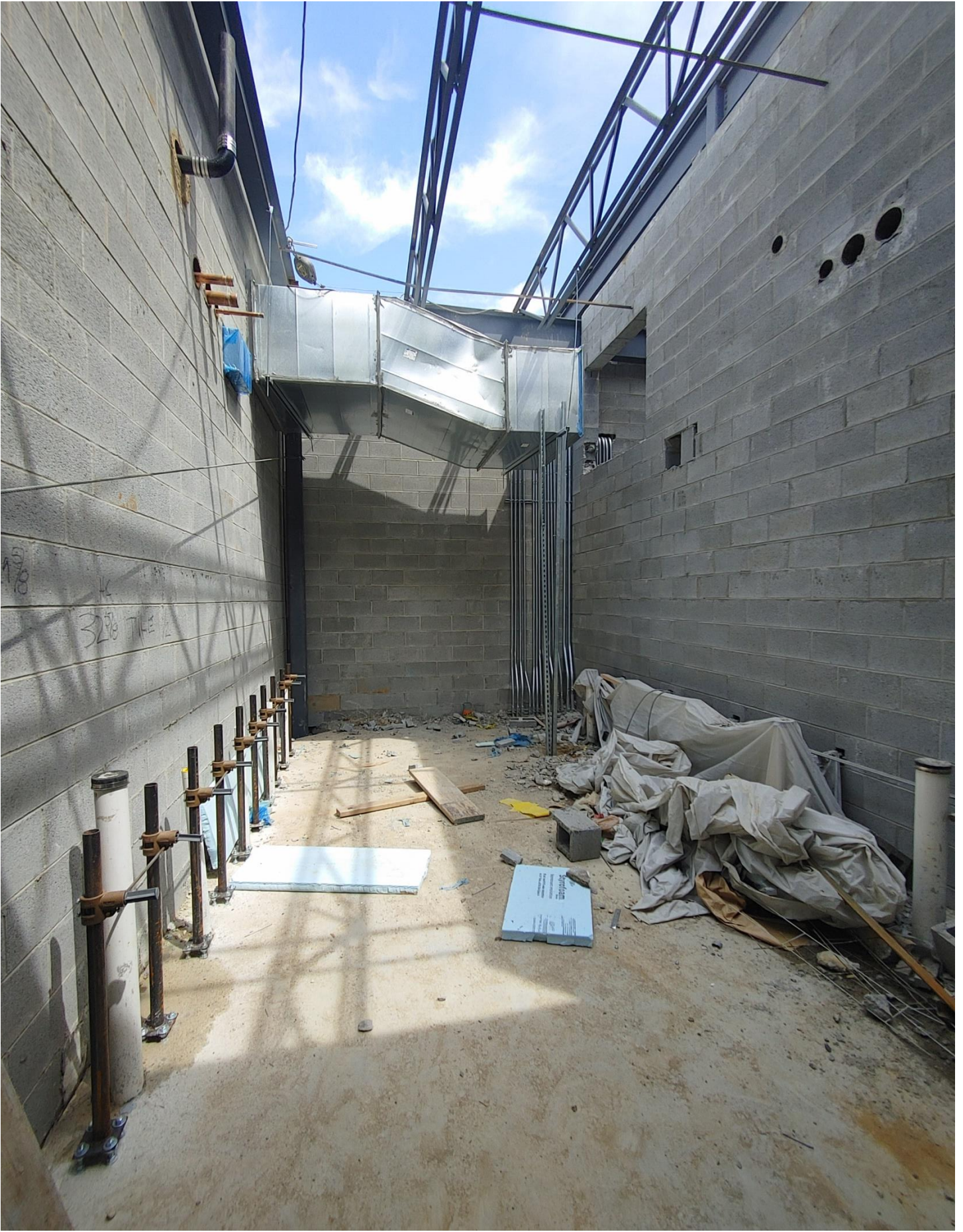
Photo 8 - HVAC Duct is being run in the Girls Toilet E104.
