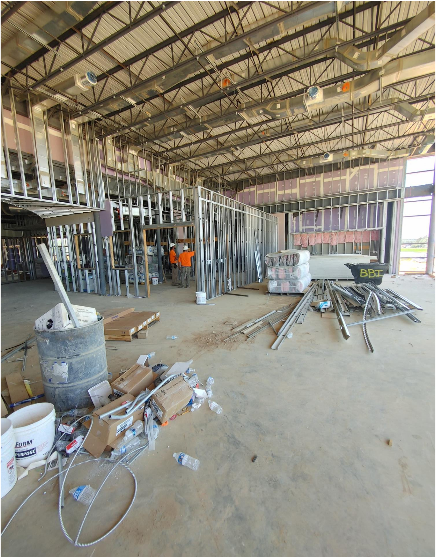
Photo 4 - Metal Stud framing continues in Area A
