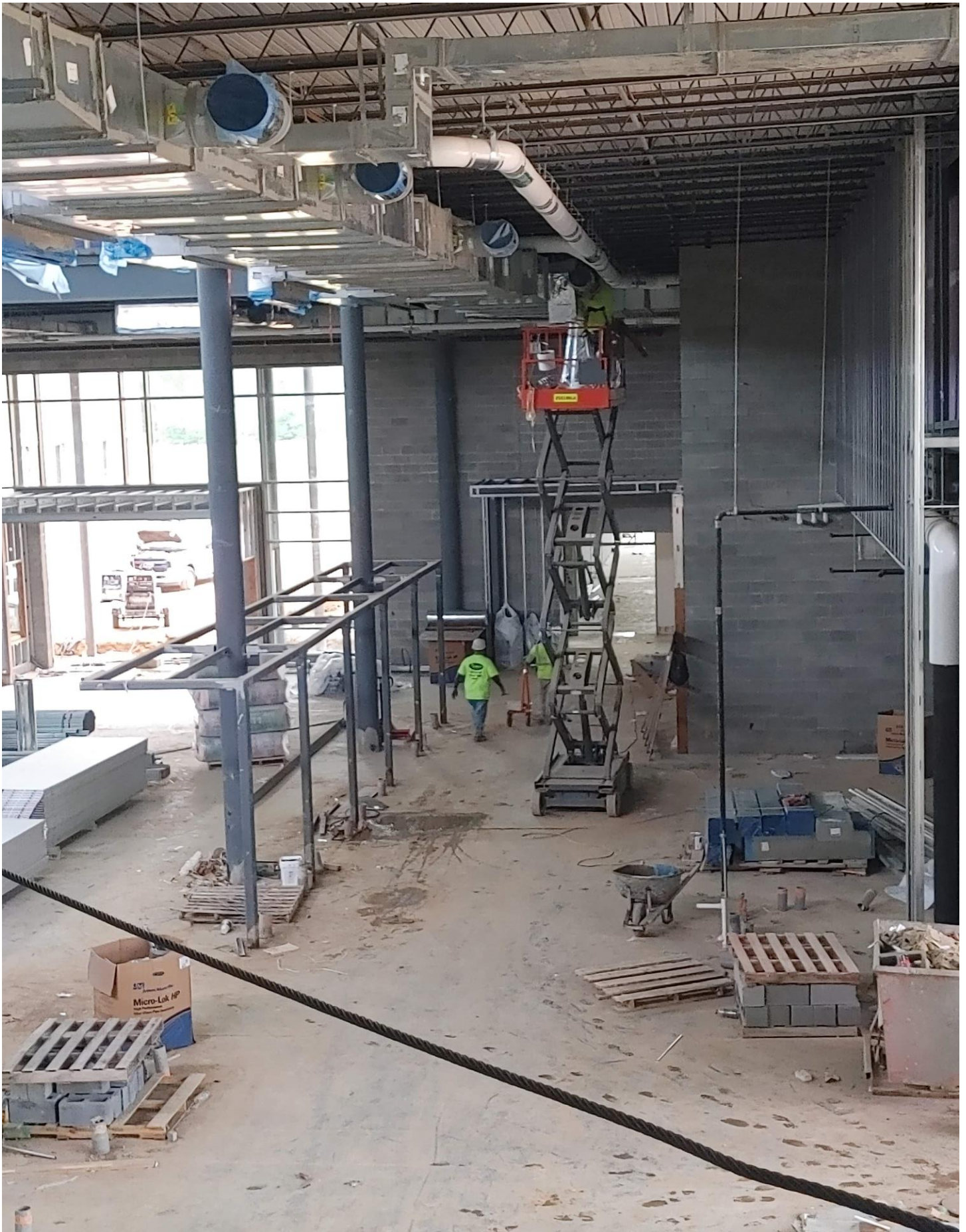
Photo 15 - HVAC Duct is being insulated in Area C.
