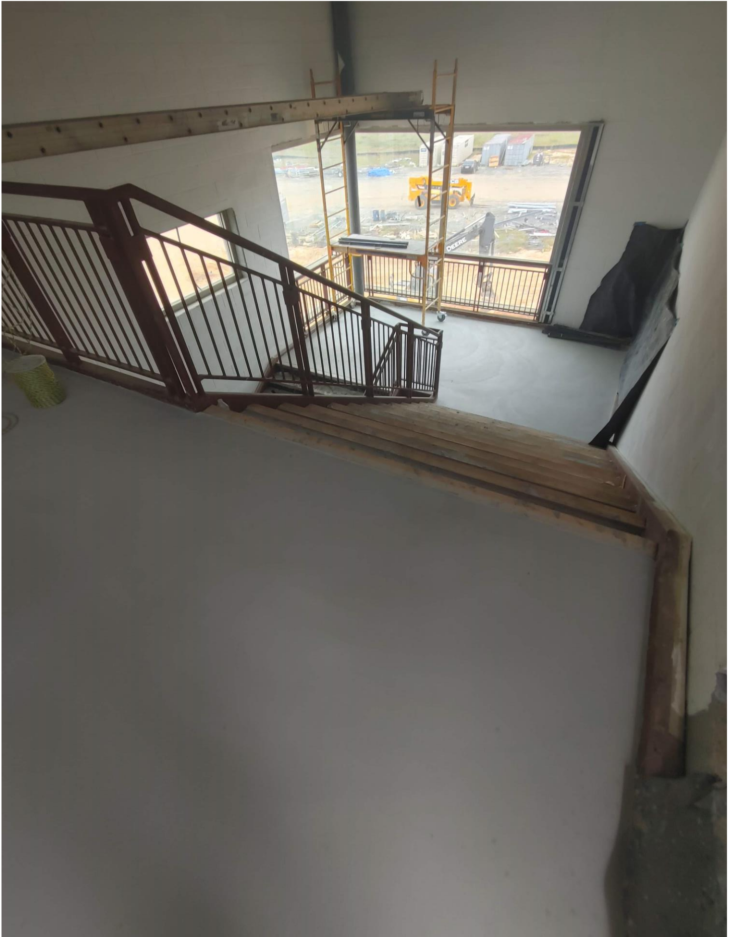
Photo 18 - All of the landings in Stairwell #2 have been poured. Two of the three landings have been poured in Stairwell #1.
