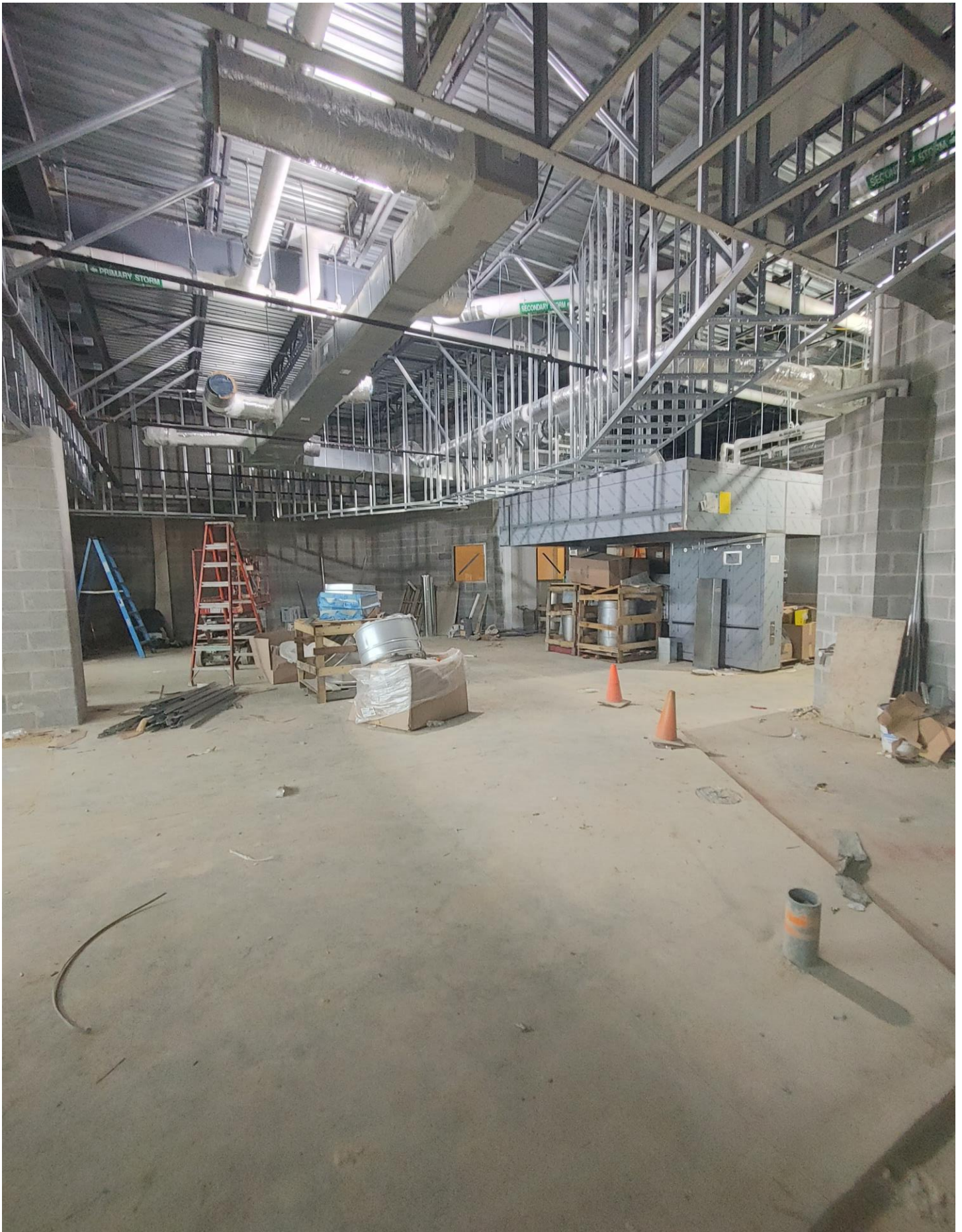
Photo 4 - Bulk Head Framing continues in the Kitchen Area.
