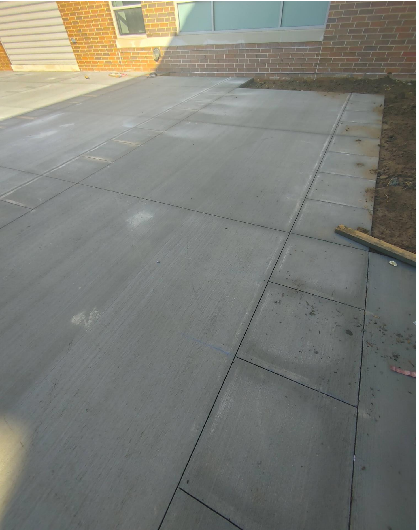
Photo 3 - Concrete is being Scored between Zone #3 & #5
